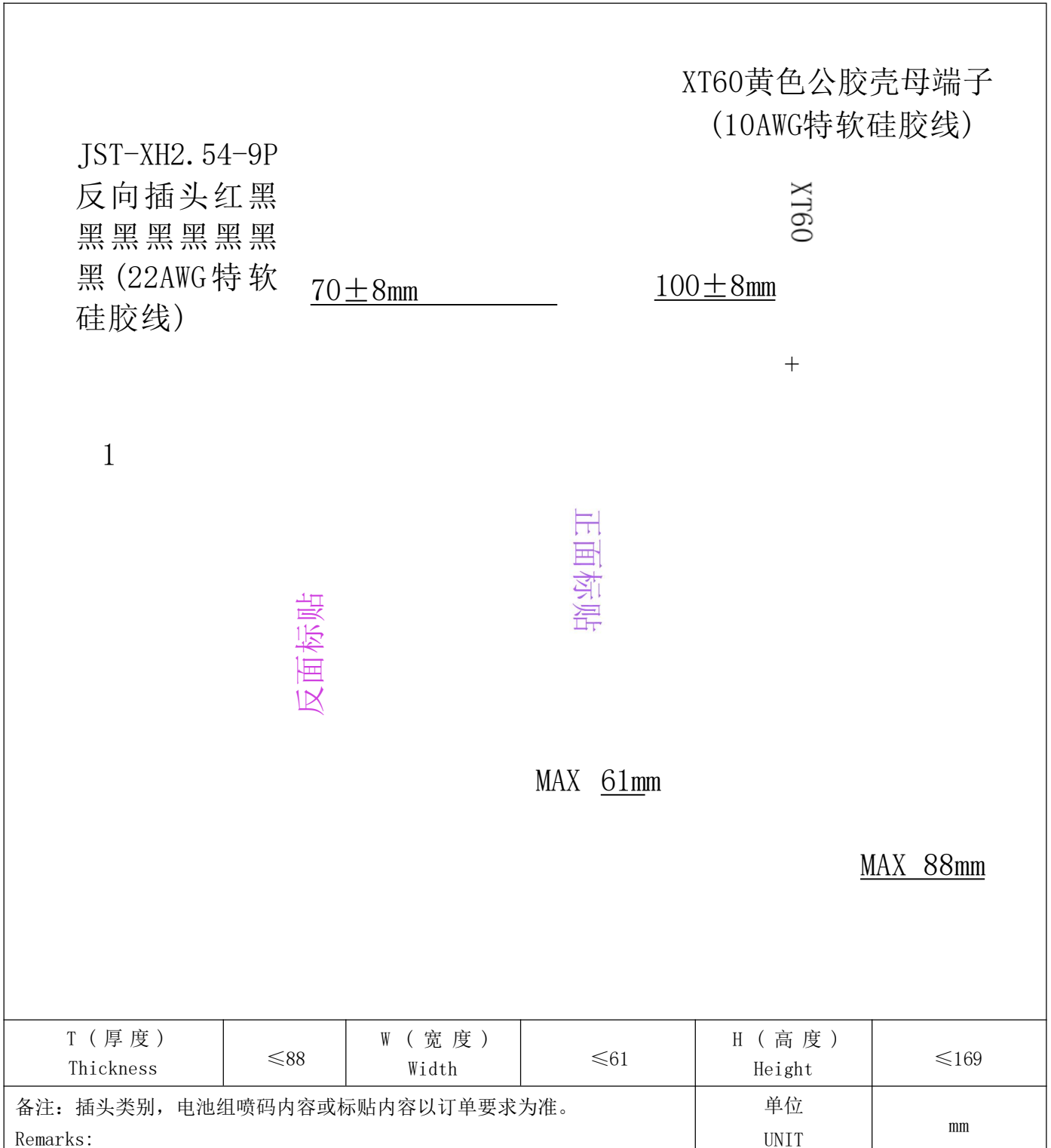
附件一：电池尺寸图 Appendix 1: Battery Dimensions Figure
